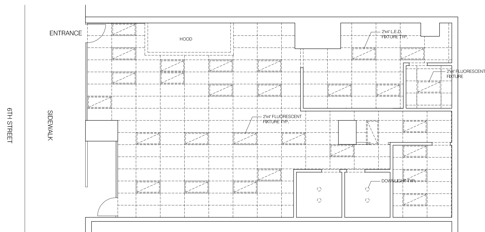
02 RCP: LIGHTING LAYOUT SCALE: 1/8" = 1'-0"
