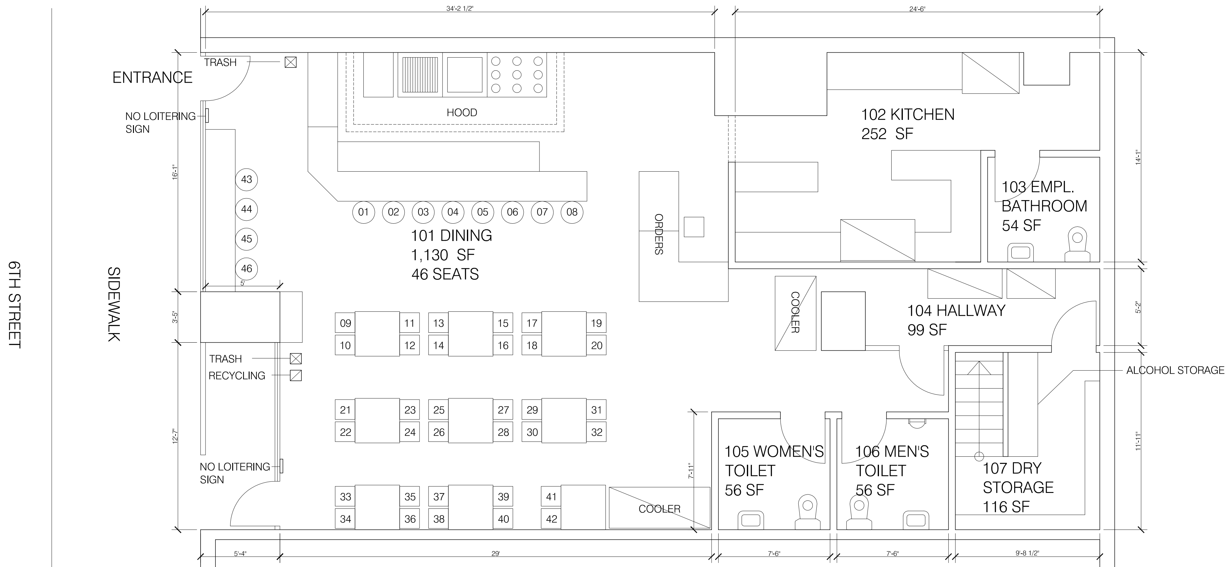
01 FIRST FLOOR PLAN SCALE: 1/4" = 1'-0"
